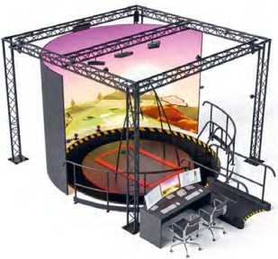
Virtual reality treadmill training. Left: Setup with treadmill, screen with integrated visual feedback for patients, cameras for precise movement analysis, and a control panel. Right: Visual feedback for patients – the white line indicates the target value of the selected gait parameter, while the red dots display the current measurements during training.
